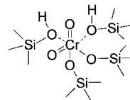
FIGURE 7. Cr attached to defect sites of silicalites.
